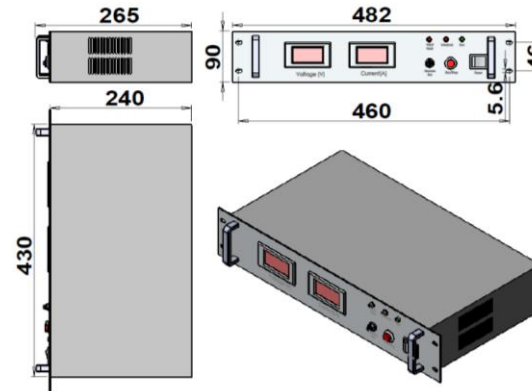
PSU-HPL-QS(12U)-3 482(L) × 265(W) × 90(H) mm 3 , 13kg
